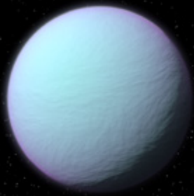
Kepler-51 b
